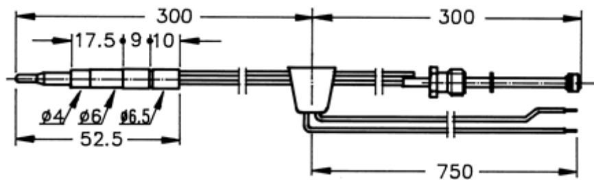
"ST" Joint - M 9 x 1 fitting - 750mm approx. cables
